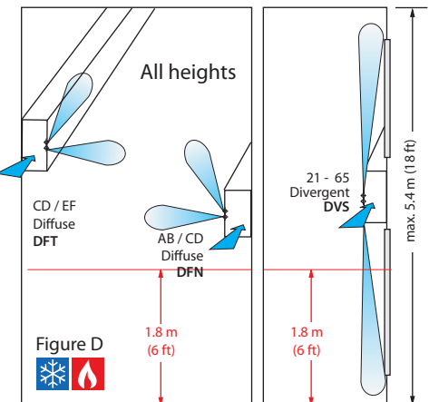
Figure D SRA diffuser with eccentric and/or nozzle rollers
